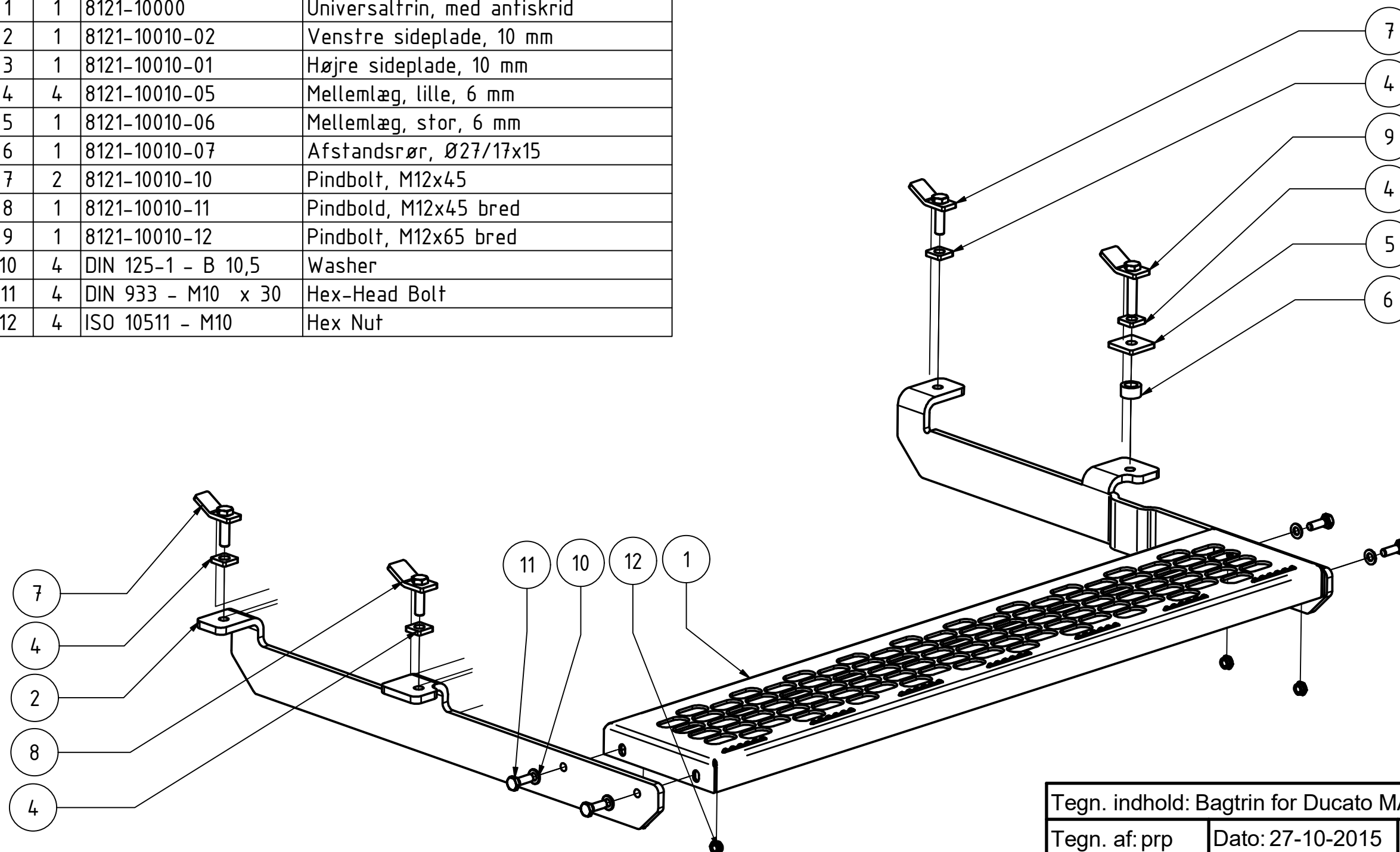
Parts List
